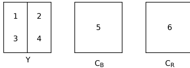
FIGURE 10/H.261 Arrangement of blocks in a macroblock
